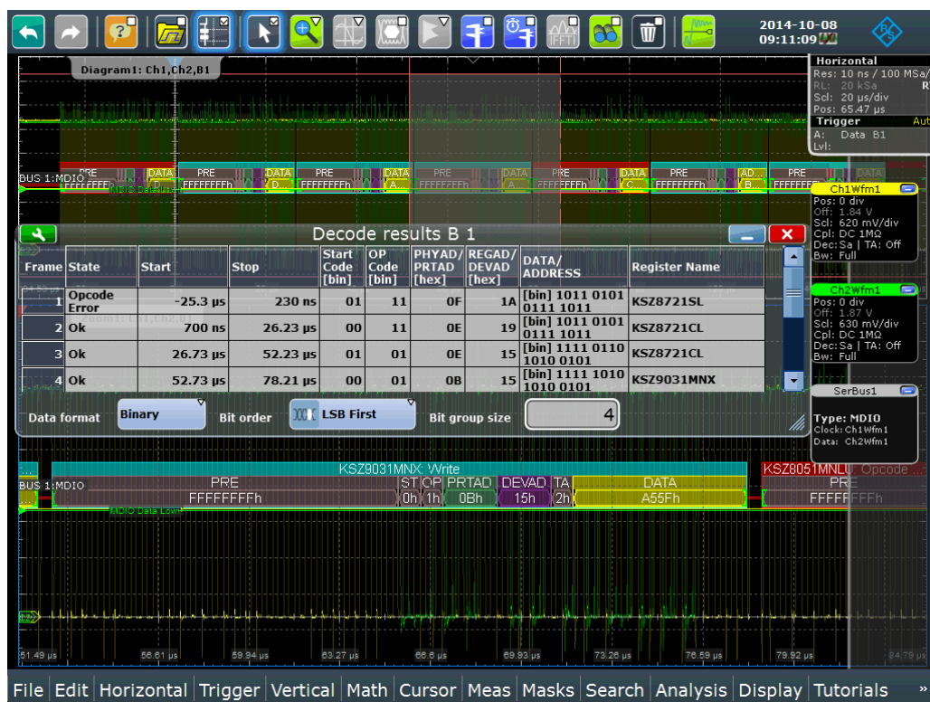
Figure 13-99: The same signal trace and decode results table as in the previous figure, but only with "DATA" in binary format
