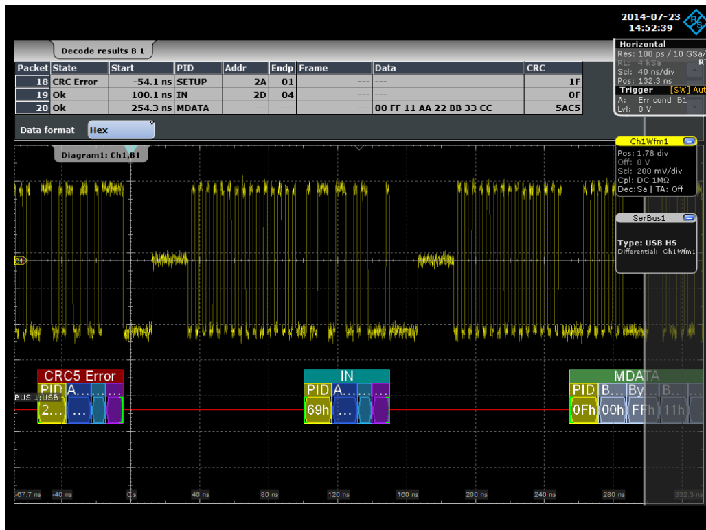
Figure 13-112: USB high speed protocol: decoded and binary signal, and decode results
