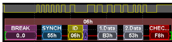
Figure 13-33: Decoded frame with checksum error (frame No 1 in figure above)
