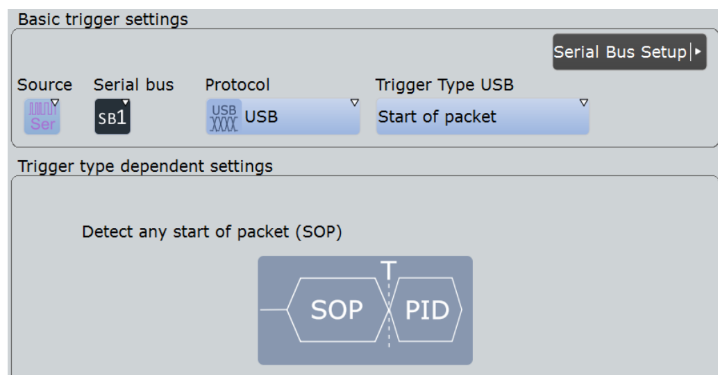
Figure 13-110: USB trigger event settings dialog
