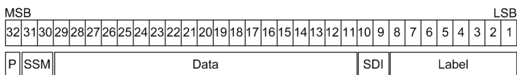
Figure 13-49: Structure of an ARINC 429 word
