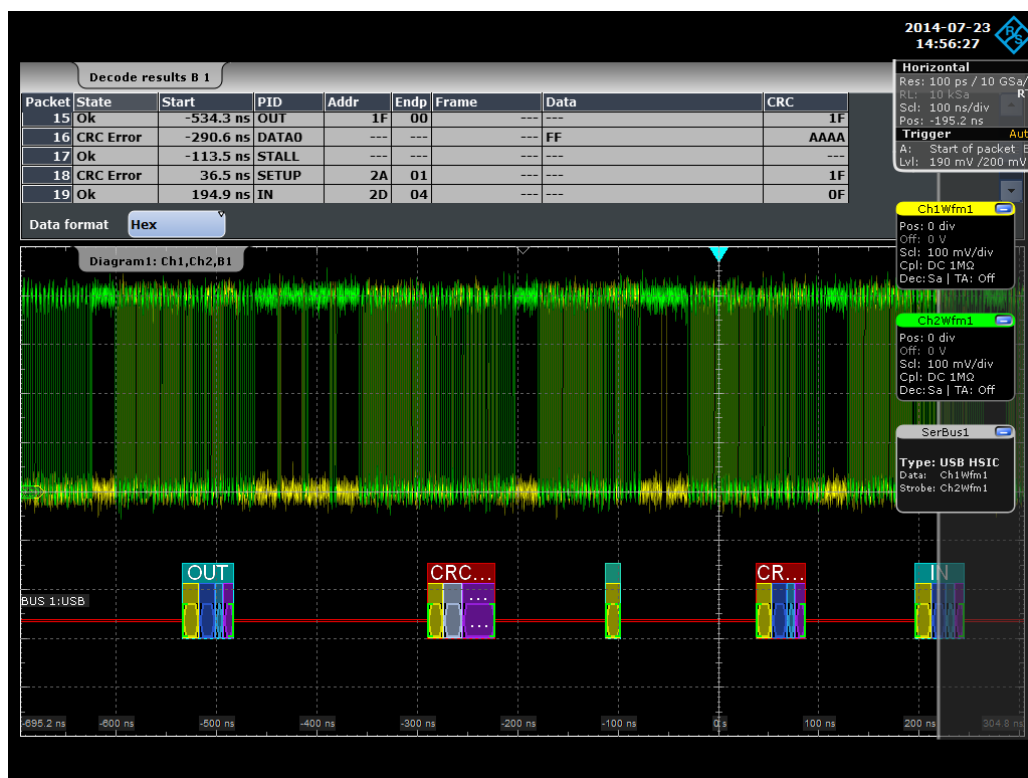
Figure 13-113: USB HSIC protocol: decoded and binary signal, and decode results
