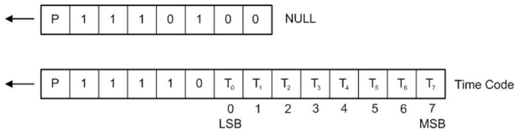
Figure 13-116: SpaceWire control codes
