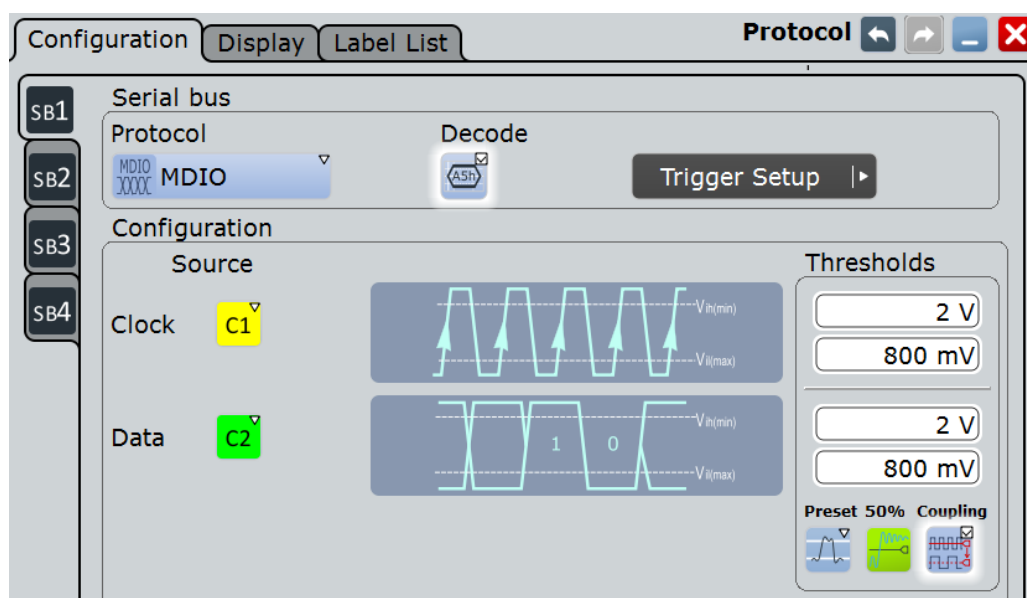
Figure 13-96: Serial bus protocol configuration dialog
