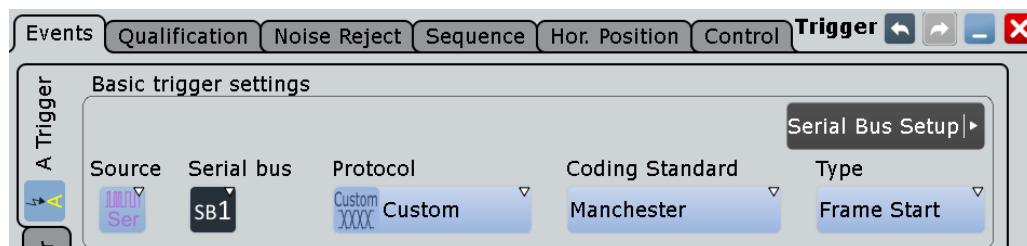
Figure 13-90: Custom serial bus trigger event settings dialog (here with "Manchester" and "Frame Start" selected)
