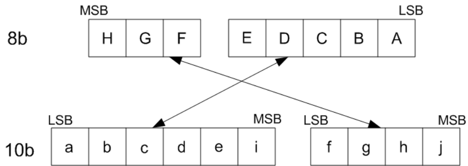
Figure 13-95: Coding scheme of the 8b/10b
