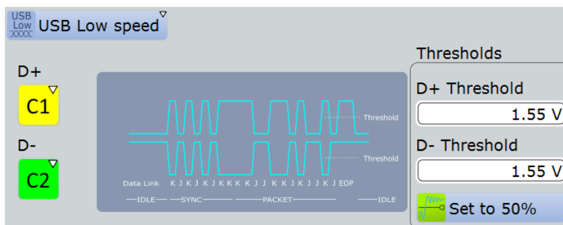
Figure 13-106: USB low speed protocol configuration
