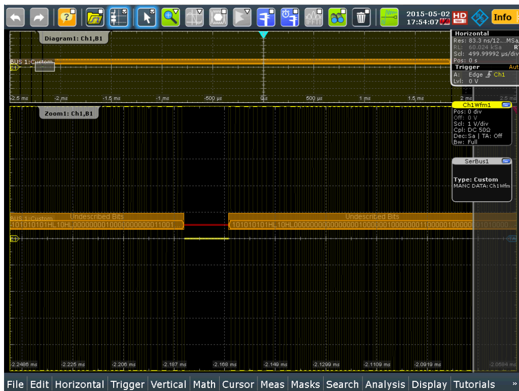
Figure 13-94: The function "Undescribed Bits" catches frames missed by the frame format descriptions
