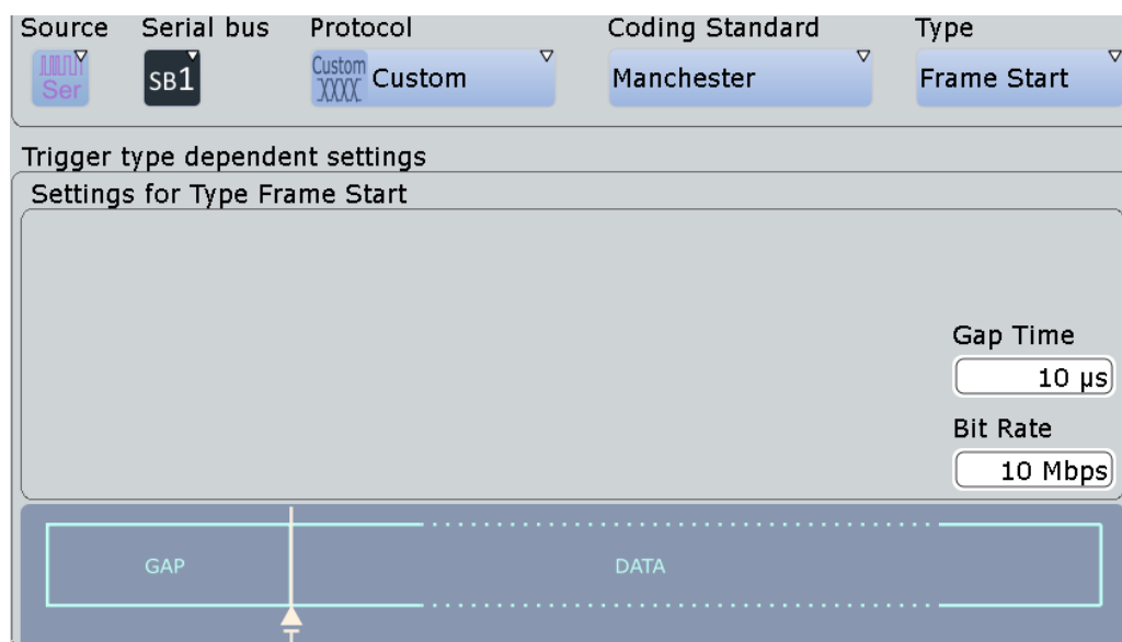
Figure 13-91: Custom serial bus dialog for setting the frame start trigger
