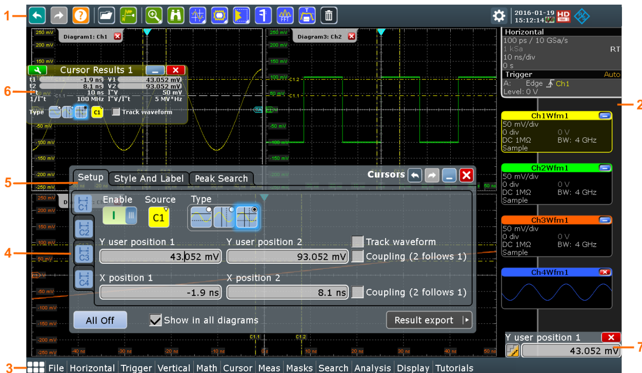
Figure 2-4: Control elements on the touchscreen
