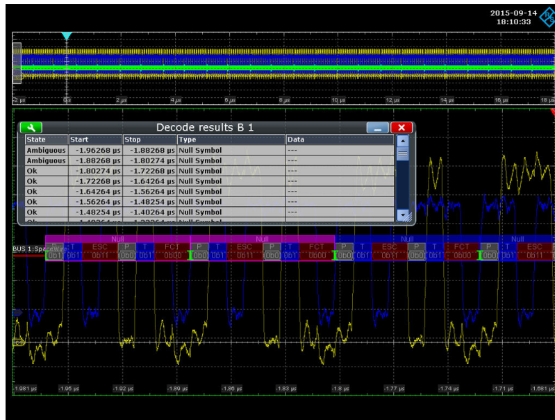
Figure 13-117: Decoded SpaceWire signal with ambiguous bits
