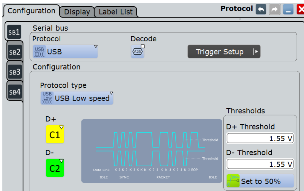
Figure 13-105: Serial bus protocol configuration dialog
