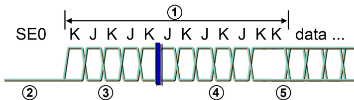
Figure 13-104: Start of a high speed packet: after an SE0, the packet starts with a SYNC field (or SOP), followed by the data packet
