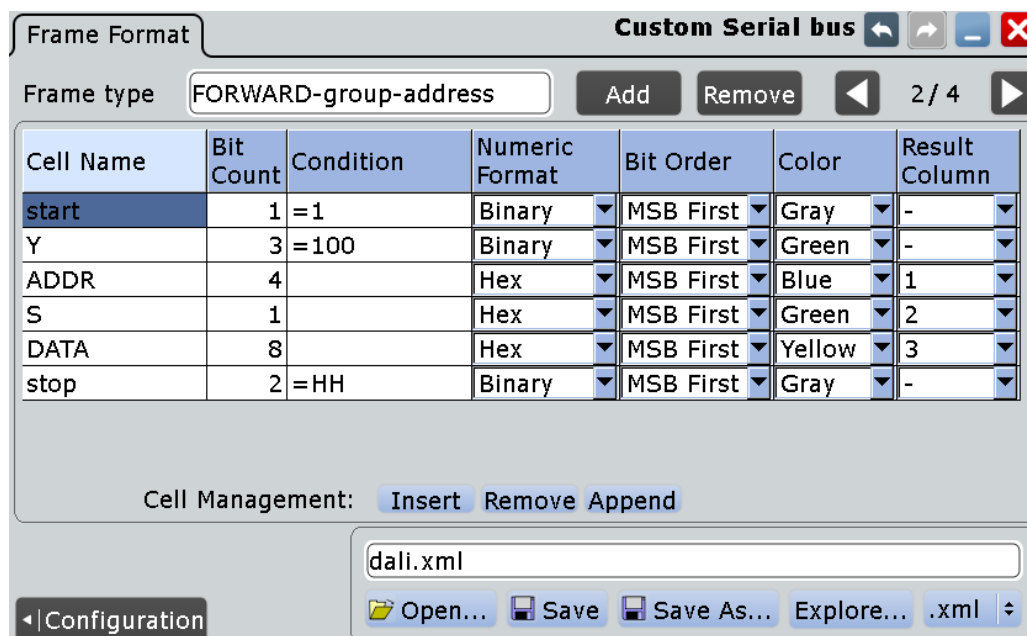
Figure 13-85: Example of a custom "DALI" frame format description (frame 2 of 4)
