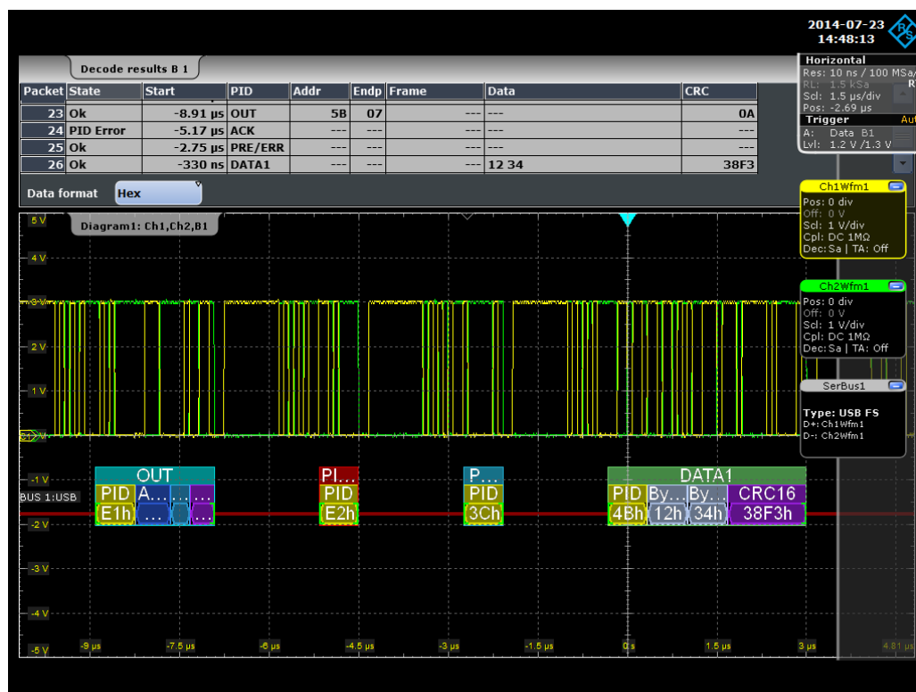
Figure 13-111: USB full speed protocol: decoded and binary signal, and decode results
