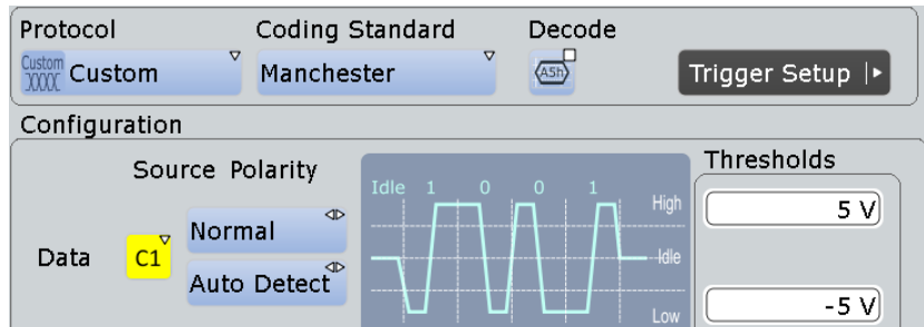
Figure 13-81: Custom serial bus coding configuration Manchester
