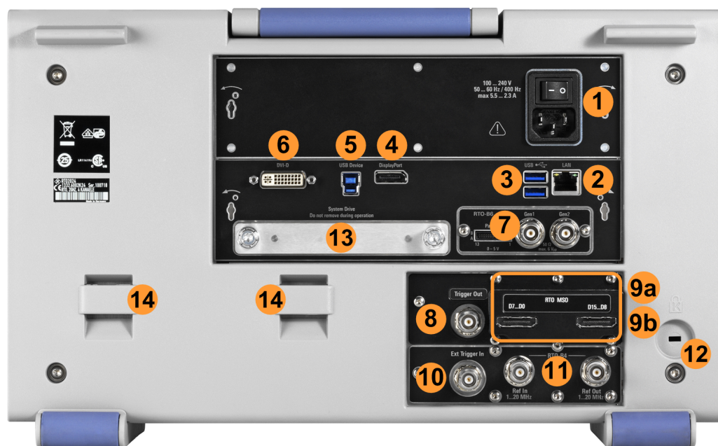
Figure 2-2: Rear panel of R&S RTO
