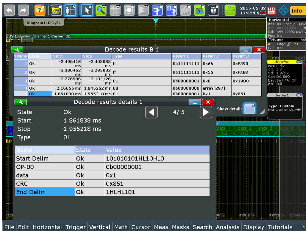
Figure 13-93: Decode results table and details of a "Profibus Voltage" protocol sample waveform
